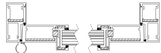
Horizontal Section UL Level 8
