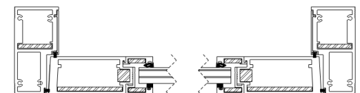
Horizontal Section UL Level 3
